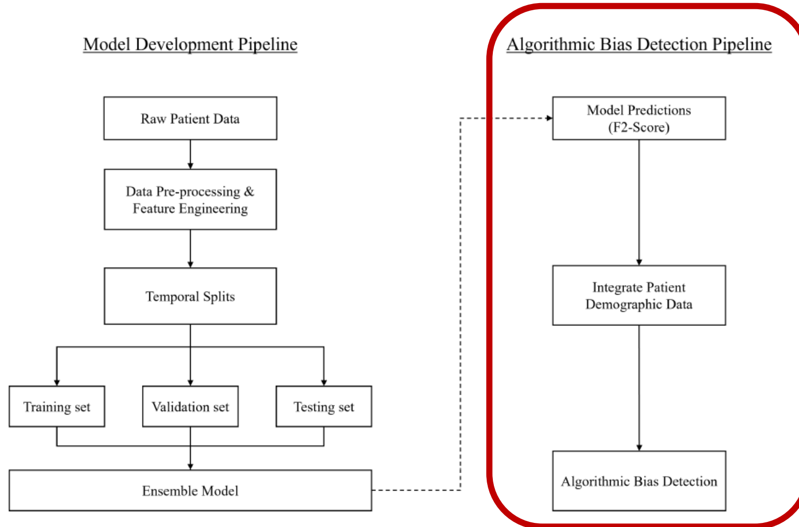
Figure 8: Algorithmic bias detection pipeline.
